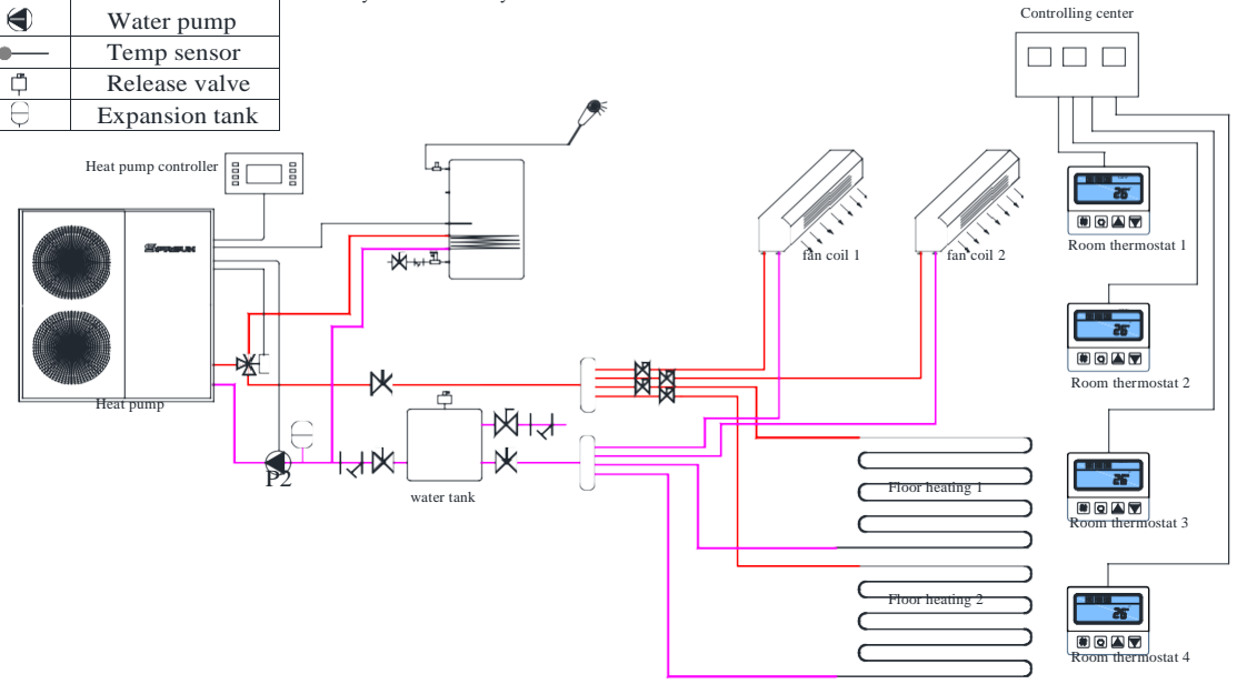
SPRSUN DC inverter air source heat pump
