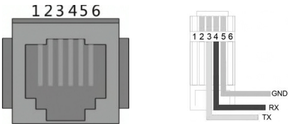
RS232 Port
